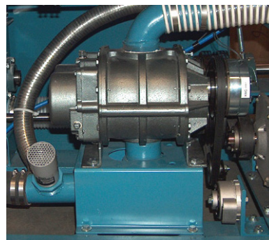
Positive Displacement Blower
